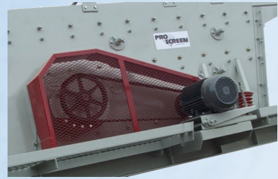
20 HP TEFC motor w/ 3 belt drive & guard.
